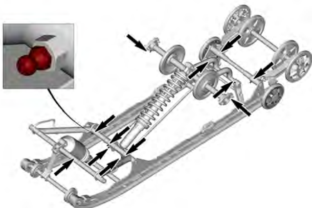
EASY RIDE+ A WITHOUT QUICK ADJUST REAR STAND
