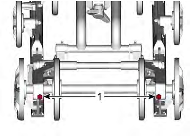
1. Adjustment screws
