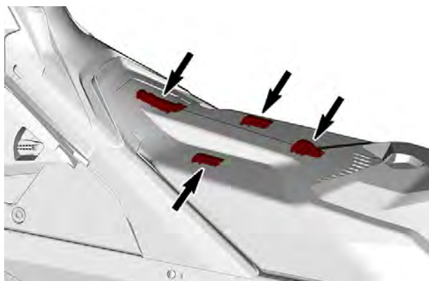
RETAINING TABS
