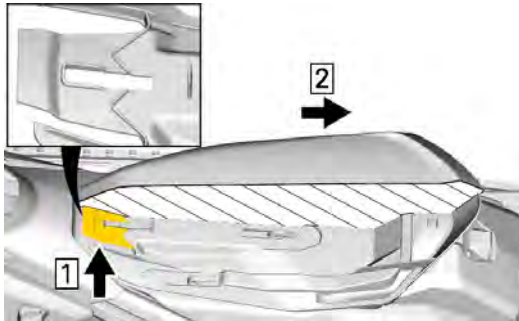
Typical — Crosscut view of seat foam
