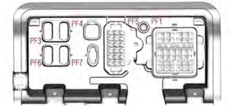
FUSE BOX SUPPORT
