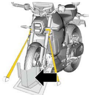
Front Wheel Lock
