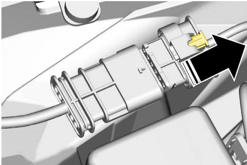
Disconnecting FRCL Connector Under Driver Seat
