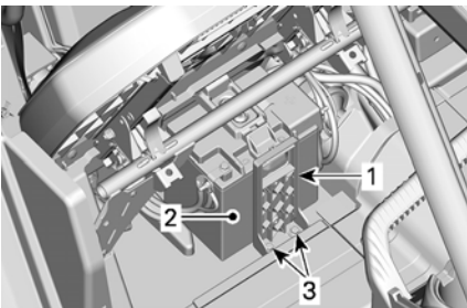
1. Battery holder
