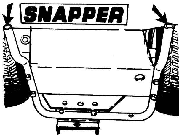
FIGURE 3-SUPPORT TUBE AWAY FROM FENDER (FOR TWIN BAG CATCHER)
