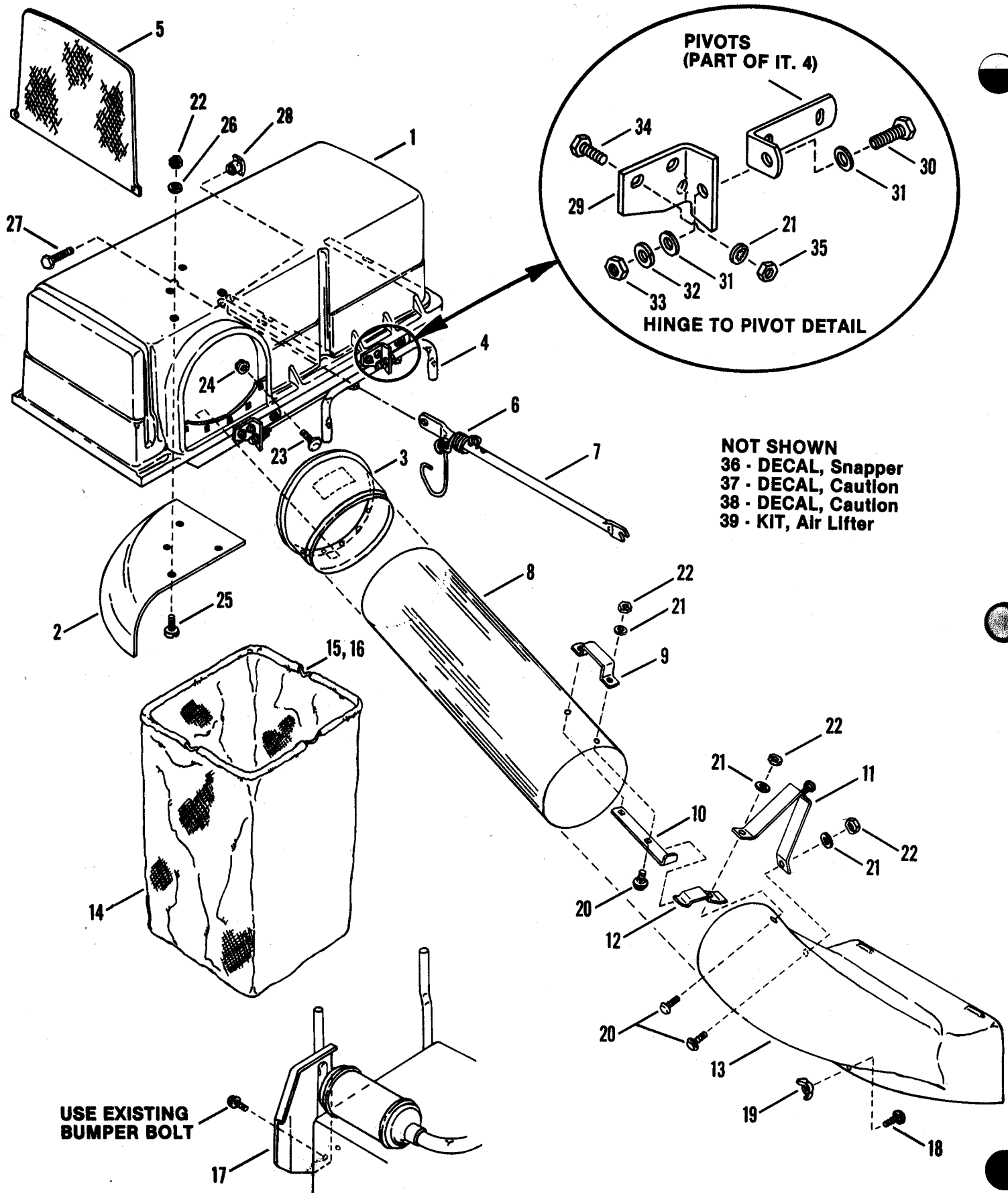
FIGURE 3 - TWIN BAG KIT COMPONENTS
