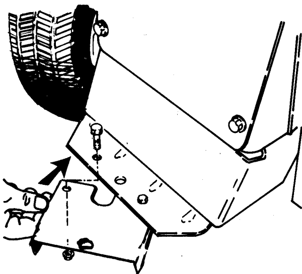
FIGURE 1-INSTALLING EXTENSION
