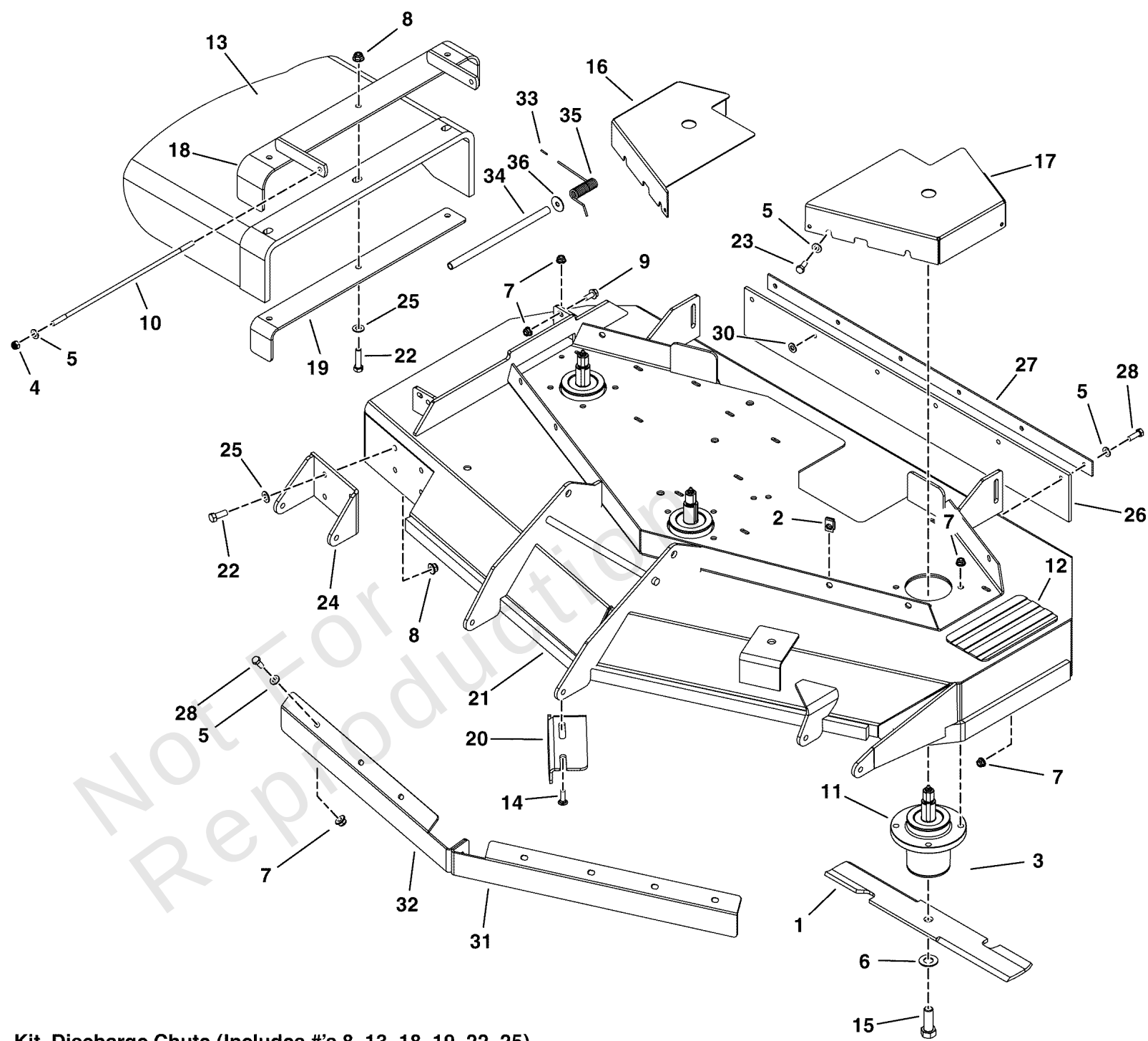
29 - Kit, Discharge Chute (Includes #'s 8, 13, 18, 19, 22, 25)
