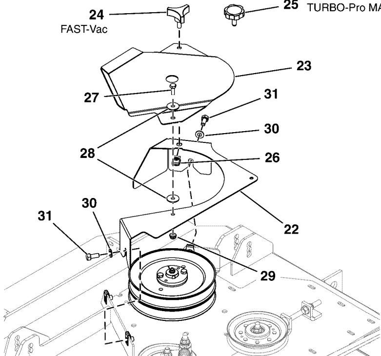
61" Mower Decks w/ Tapered Hub (5304153, 5304154) TURBO-Pro / TURBO-Pro MAX
