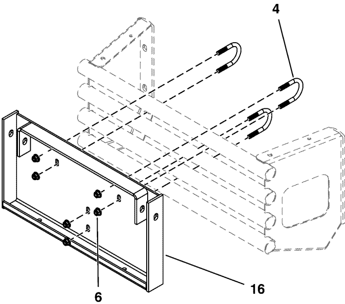
Round Tube Bumpers (IS3100Z Models) 5303942
