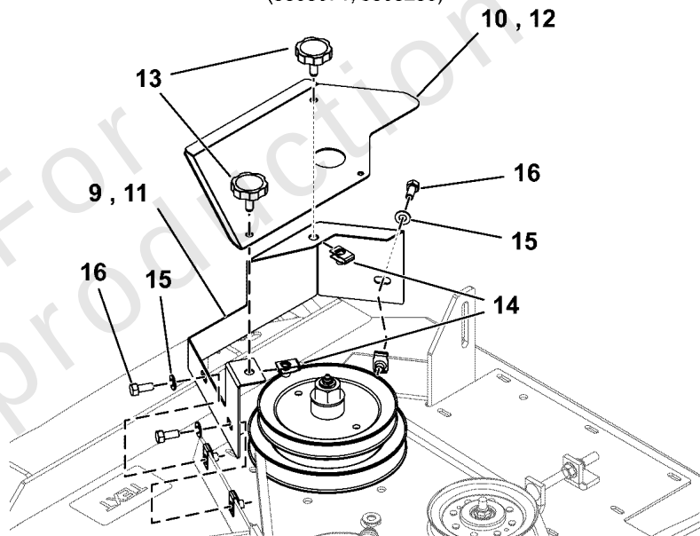
Mower Deck Guards (5303071, 5303259)
