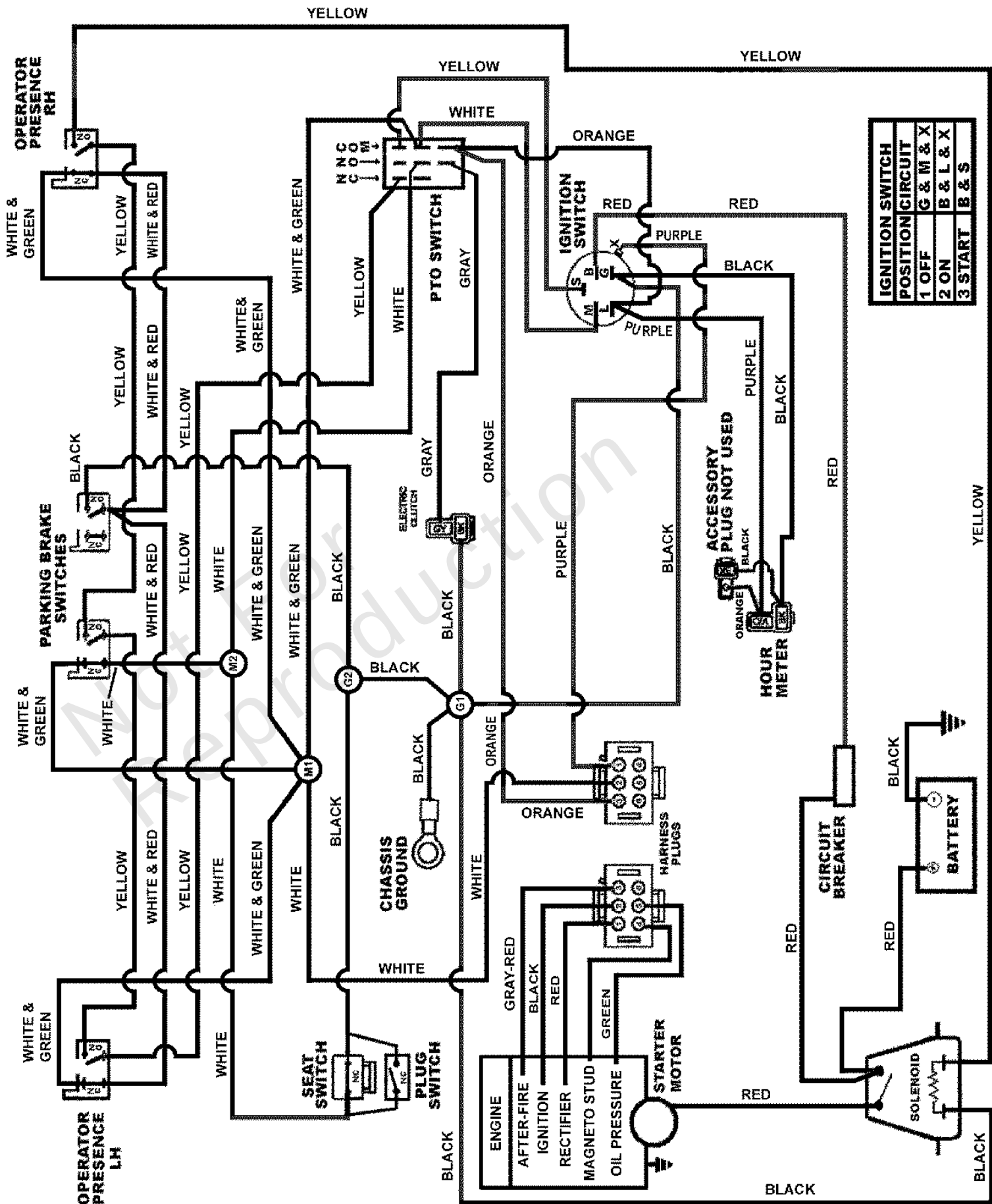
WIRING SCHEMATIC for ZT20500BV HARNESS Part #5048640
