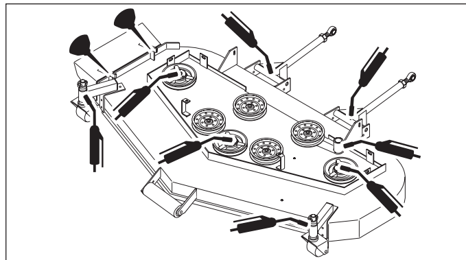
Figure 21. Deck Lubrication
