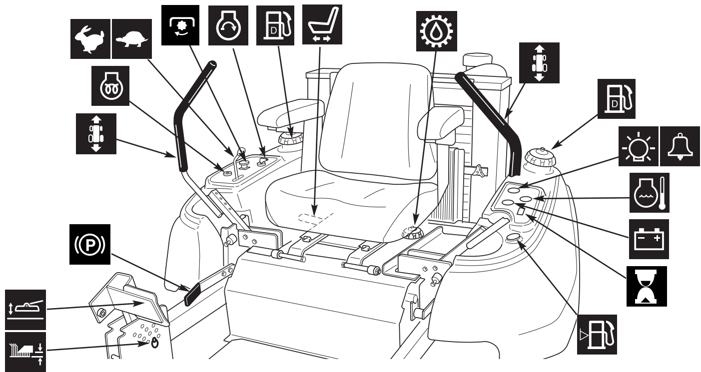
Figure 1. CONTROL FUNCTIONS
