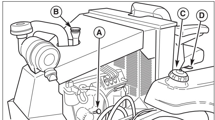
Figure 2. Pre-Start Checks
