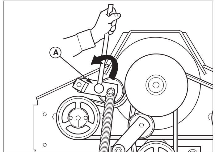
Figure 53. Pump Belt Removal & Replacement
