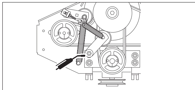
Figure 23. Gearbox Drive Idler Pivot
