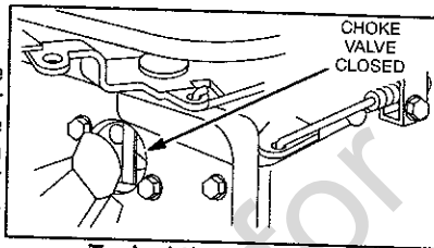
Typical throttle control
