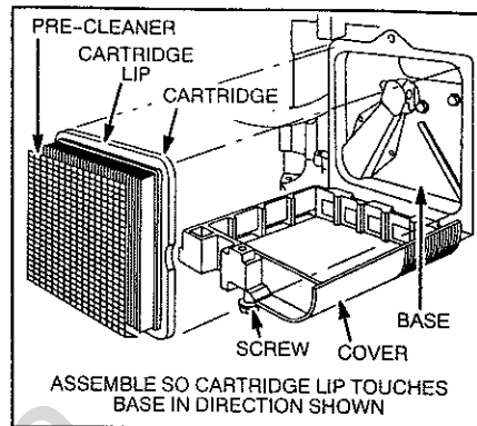
Dual element air cleaner
