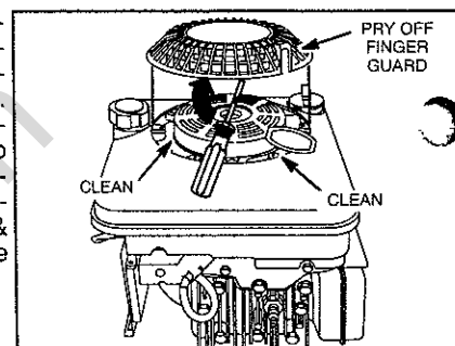
Cooling system
