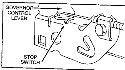
Stop switch check
