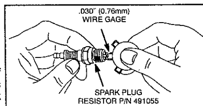
Spark plug
