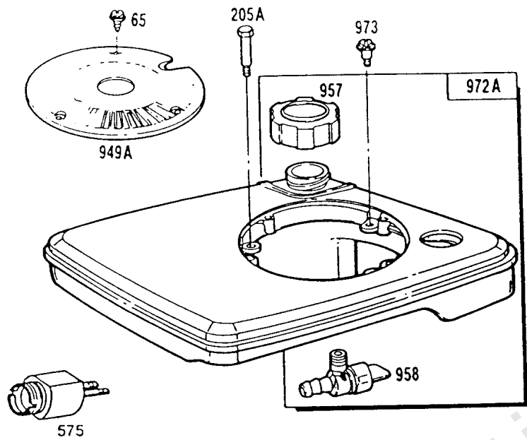
REF. 972A FUEL TANKS FOR ENGINES WITH VERTICAL PULL OR ELECTRIC STARTERS
