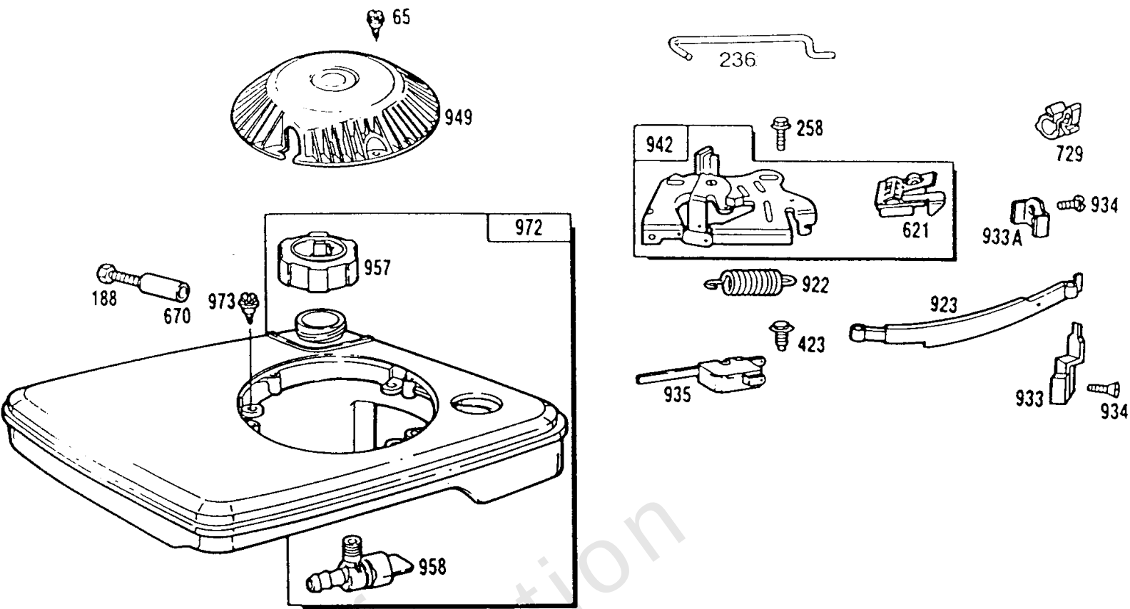
REF. 972 FUEL TANKS FOR ENGINES WITH REWIND START ONLY
