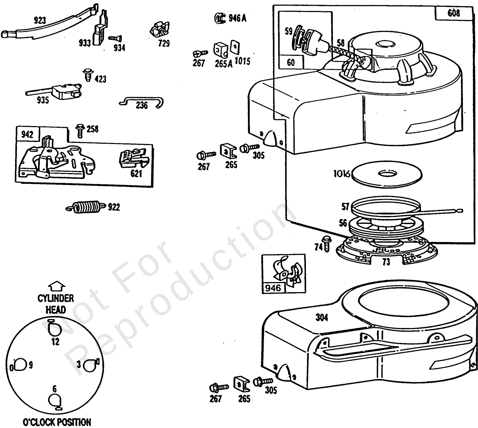
REWIND STARTER ASSEMBLIES WITHOUT BAND-BRAKE CLOCK POSITIONS
