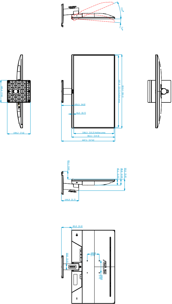
ASUS VA27EHF2 Outline Dimension * Unit: mm [inch]
