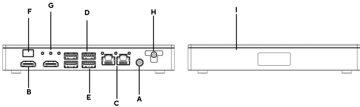
Figure 4. Slim Chassis Layout – NUC 13 Rugged Kit
