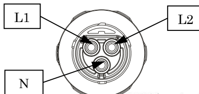
Male Connector
