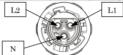
Female Connector
