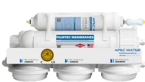
1 RO system head with pre installed membrane
