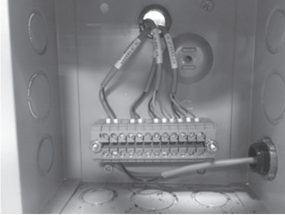
Figure 33. Boiler Terminal Strip
