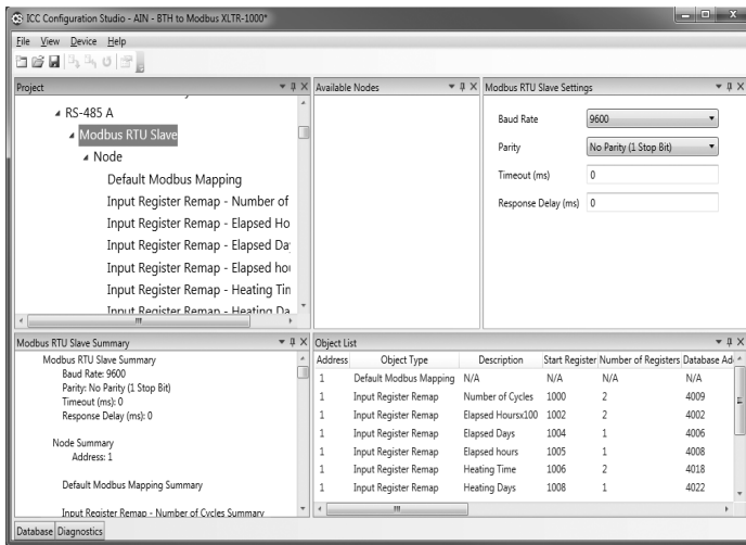
Figure 2. Changing ModBus Parameters
