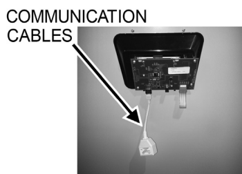
Figure 28. Reconnecting RJ45 Plug from Split Communication Cable
