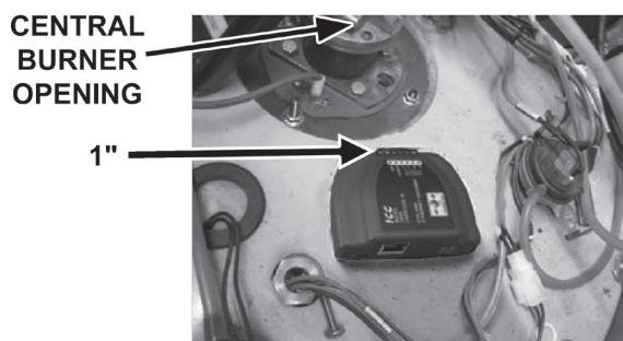
Figure 25. Connecting the Communications Cable to the Module
