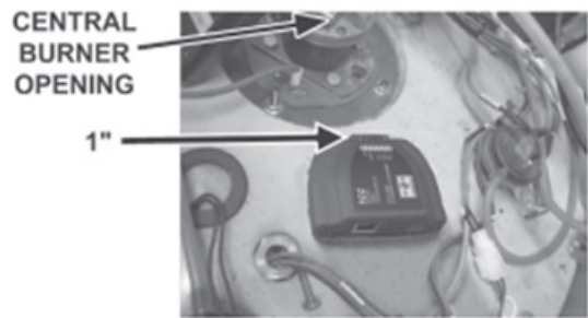
Figure 16. Clearance of ICC Unit from Central Burner Opening
