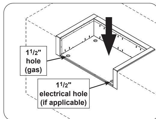
Fig. 3-3 Install insulating liner
