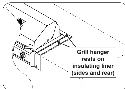
Fig. 3-4 Install grill into liner
