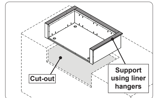
Fig. 1-1 Installation orientation
