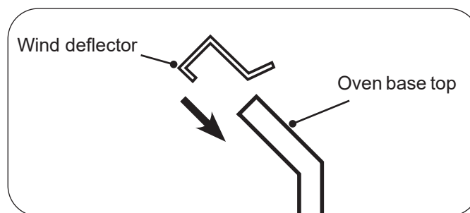
Fig. 1-3 Side view detail
