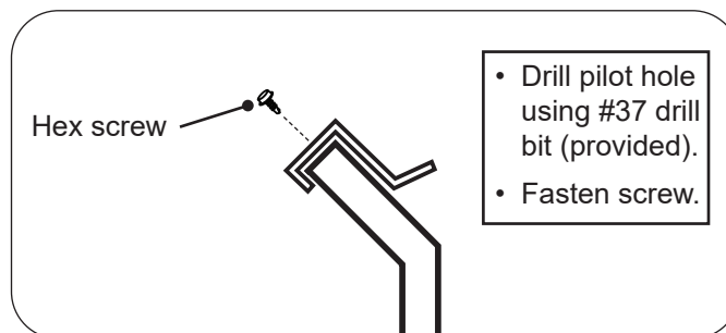
Fig. 1-4 Secure wind deflector using screw
