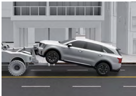
FWD vehicle
