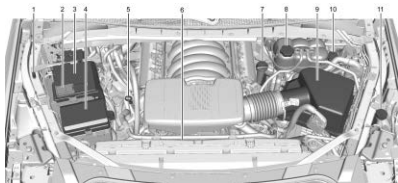
6.2L V8 Engine (L87)
