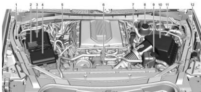
6.2L V8 Supercharged Engine (LT4)
