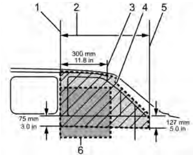
Roof-Rail Side Impact Airbag Deployment Zones – Passenger Side Shown, Driver Side Similar (Cargo Van and Cutaway Models)
