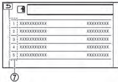
List screen
