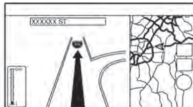
Navigation screen
