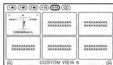
CUSTOM VIEW 5
