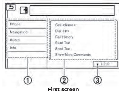
First screen
