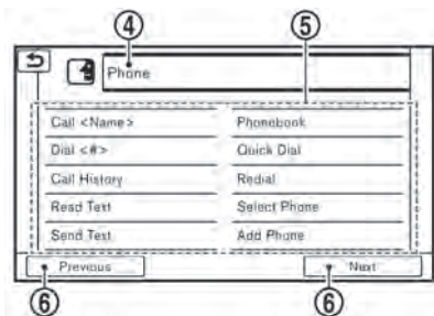
Second screen
