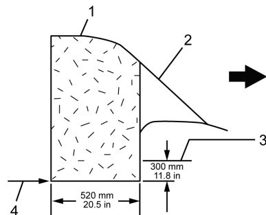
Passenger Side View of the Instrument Panel and Approximate Deployment Area of the Airbag Zone
