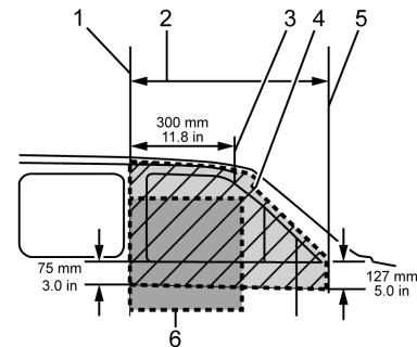
Roof-Rail Side Impact Airbag Deployment Zones – Passenger Side Shown, Driver Side Similar (Cargo Van)
