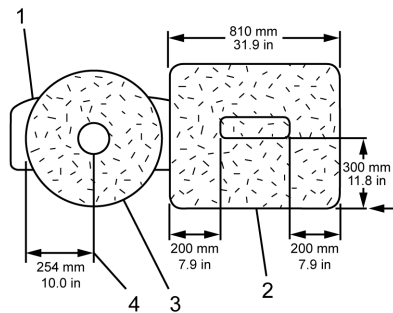
Rear View of the Instrument Panel and Approximate Deployment Area of the Airbag Zone
