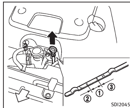
VQ35HR engine
