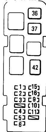
Engine compartment (left)—Canada
