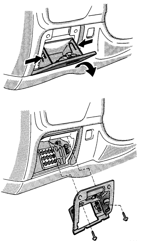
Instrument panel
